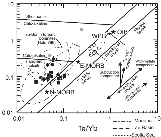
Figure 6. Th/Yb-Ta/Yb diagram from Pearce (1982) (Fig. 5 for key to symbols). Normal (N) mid-ocean-ridge basalt (MORB), enriched (E) MORB, and ocean-island basalt (OIB) normalizing values are from Sun and McDonough (1989). WPG— within-plate granite (from Harris, 1983). Fields for Mariana and Lau were compiled by Harper (2003a; their Fig. 7, p. 219), and Scotia Sea is from Leat et al. (2000). Field for Hole 786 boninites is from Murton et al. (1992).
